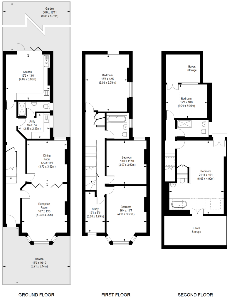
GROUND FLOOR
